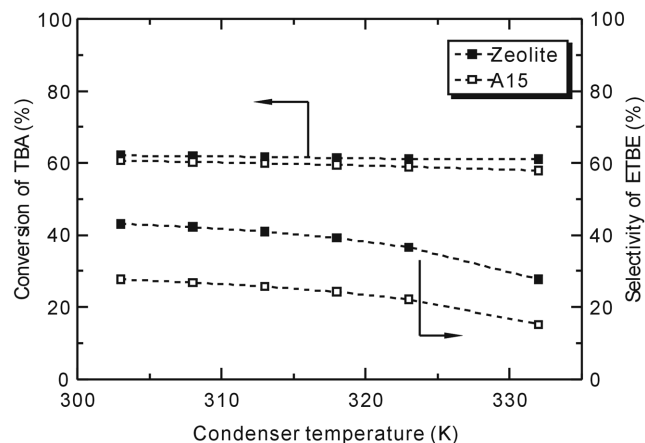
Fig. 8. Simulation results for the effect of the condenser temperature on conversion of TBA and selectivity of ETBE.
